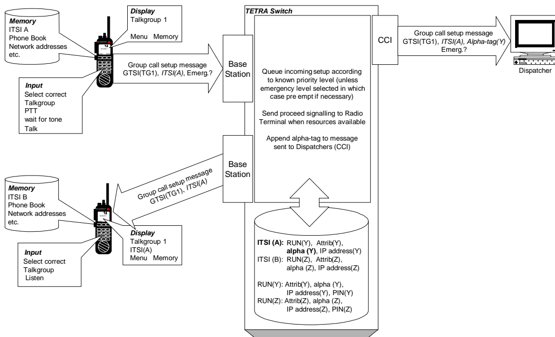
Figure B.5: Information flows for a group "speech item" originating from a Mobile Station
